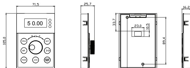
Shuttle type operation panel (SY8600-DP01)
